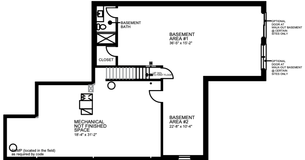
OPTIONAL FINISHED BASEMENT
