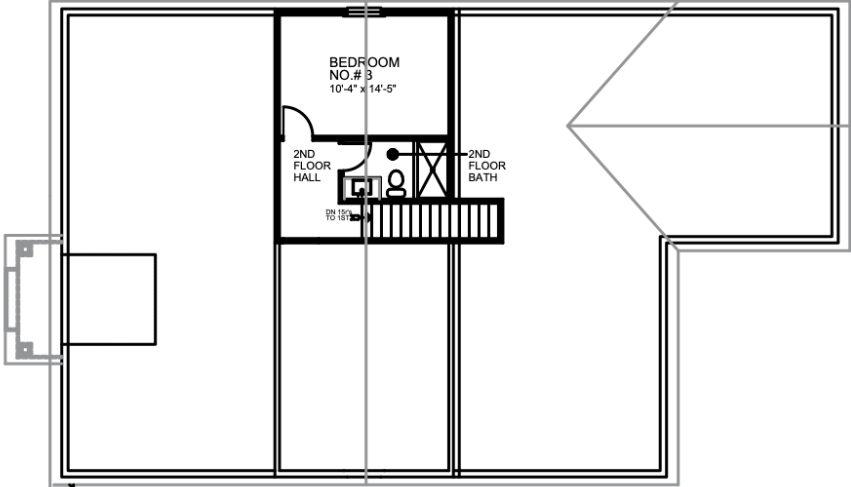
OPTIONAL SECOND FLOOR PLAN
