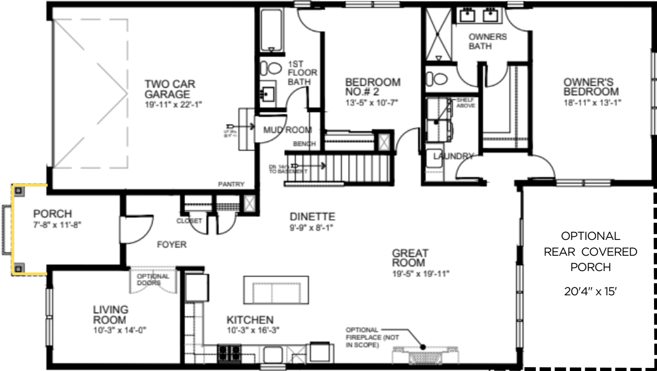
FIRST FLOOR LAYOUT WITH OPTIONAL SECOND FLOOR
